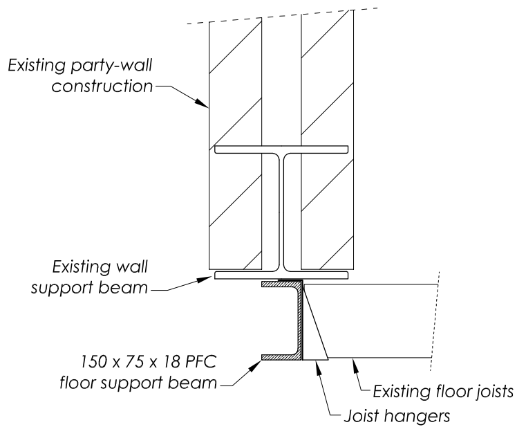
Floor Beam Detail
